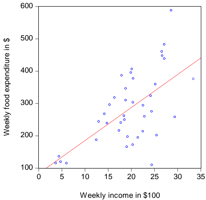
Figure 2. Scatter Diagram with Regression Line
